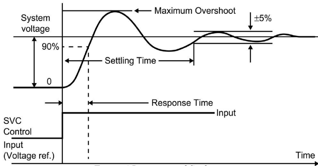
Figure-4 Response and Settling time
