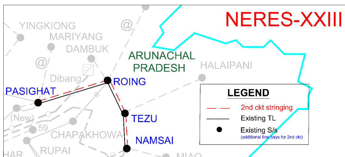
Figure 8-1: Schematic NERES-XXIII
