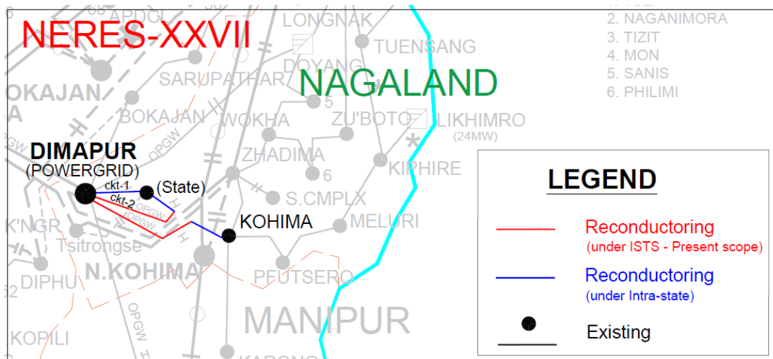
Figure 8-4: Schematic NERES-XXVII
