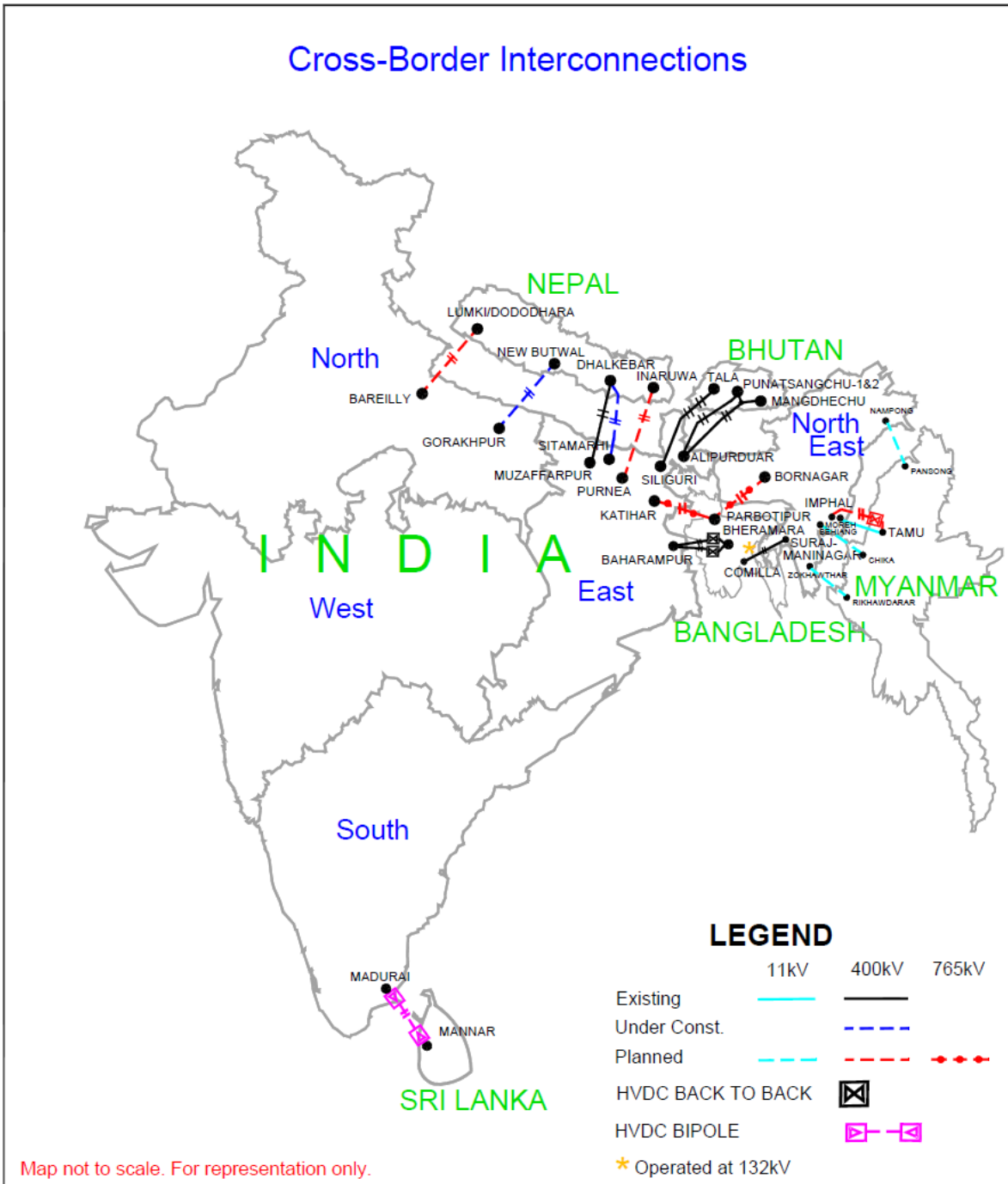
Figure 9-1 Cross-Border interconnections
