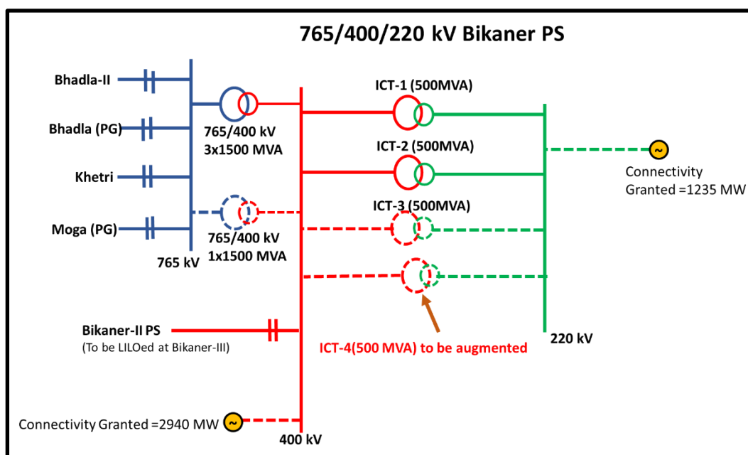
Figure 4-10: Schematic of 765/400/220 kV Bikaner PS
