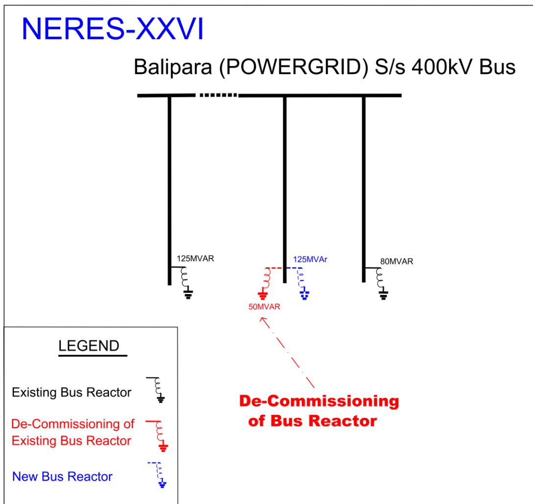
Figure 8-2: Schmeatic NERES-XXVI
